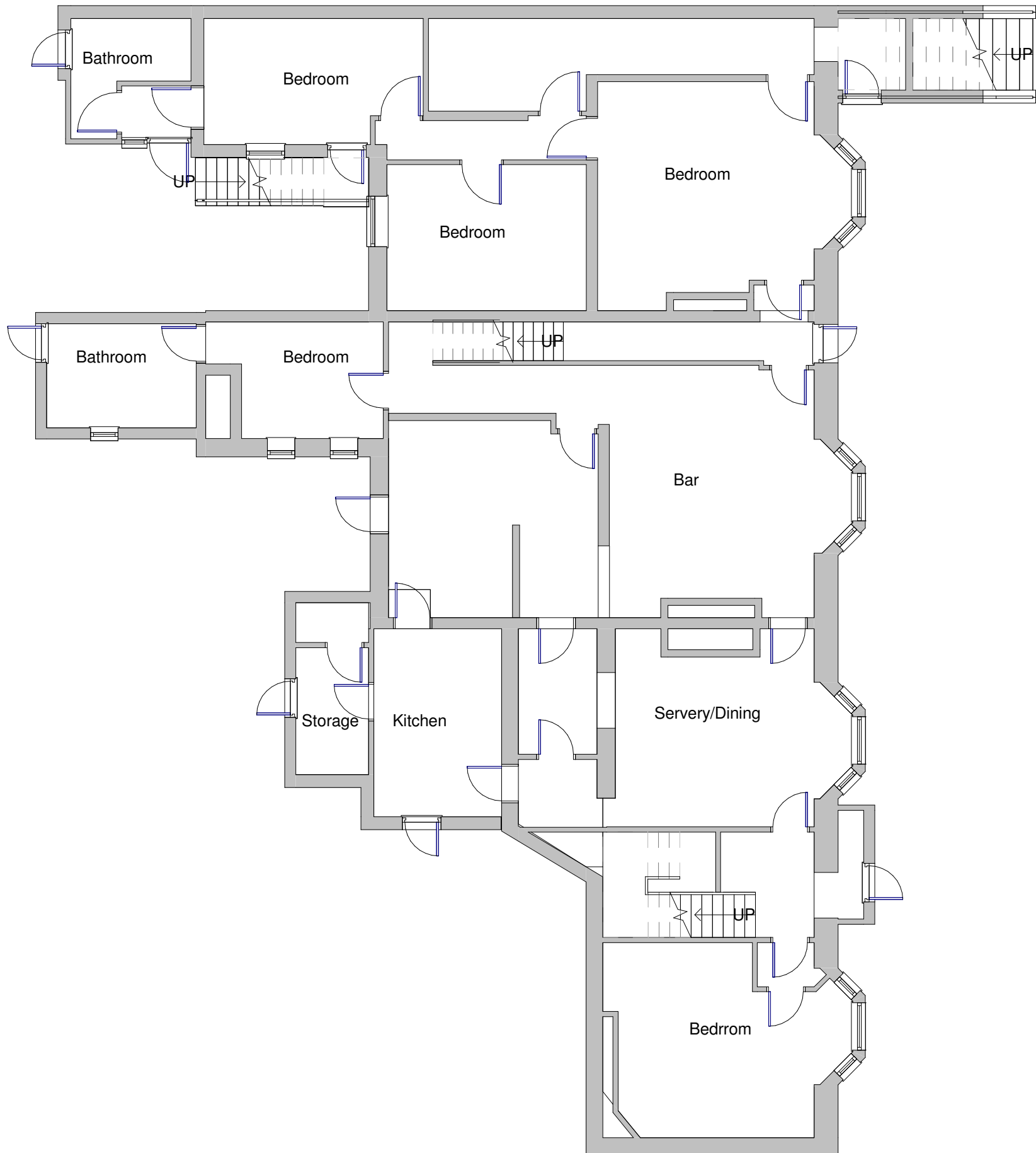
Ground Floor 1 : 100
